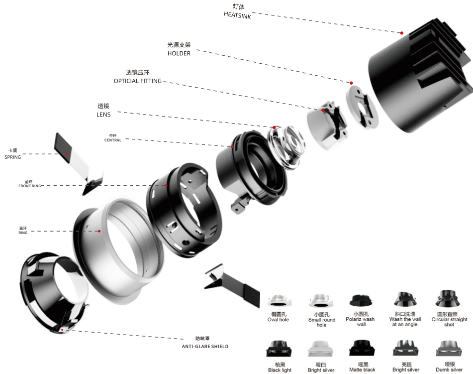
产品分解实物图 Product Breakdown Diagram
